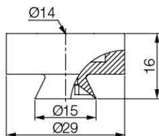
[Rubber Part]
