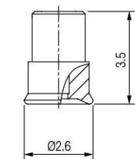
[ Rubber part ]
